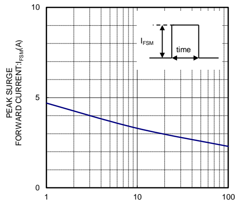
I_{FSM} - t CHARACTERISTICS
