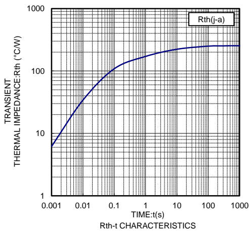
R_{th} - t CHARACTERISTICS
